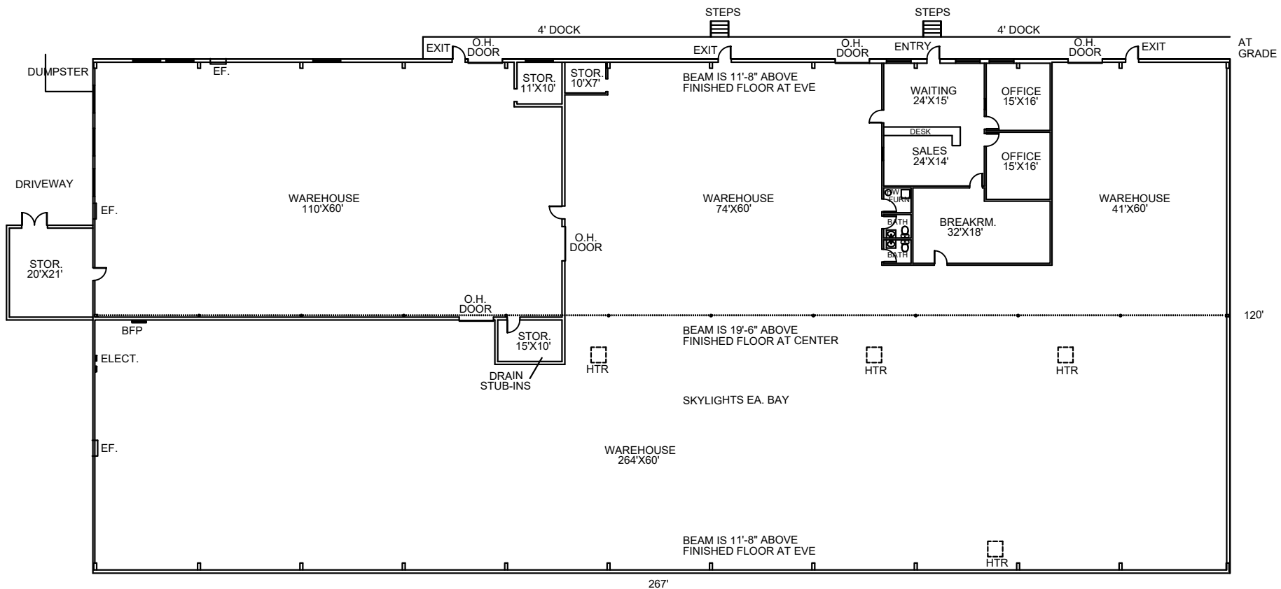
NORTH 3300 RANGELINE ST. 32,480 SF FLOOR PLAN SCALE: 3/32"=1'-0" 24X36 REVISED 10-22-24
