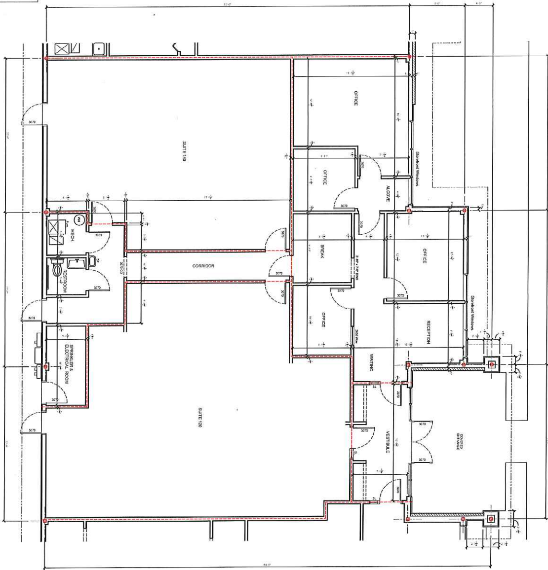
EXISTING FLOOR PLAN SCALE: 1/8" = 1'-0"
